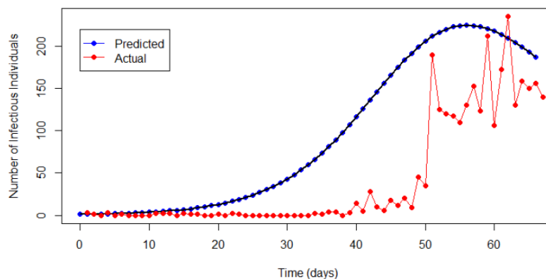
Figure 1: Actual vs Predicted Infectious Counts Trend
