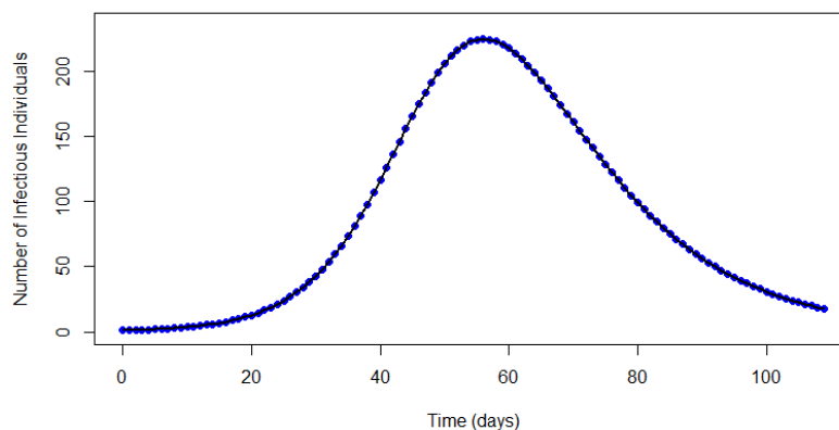
Figure 2: 110 Days Trajectory of Infectious Counts
