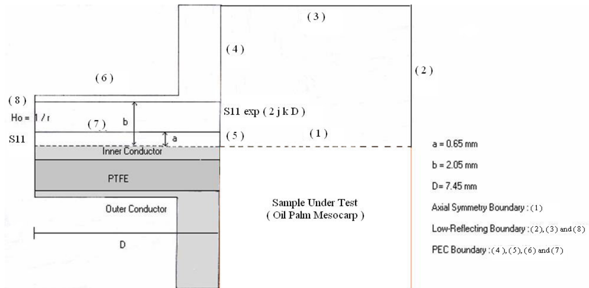
Figure 2: Rotationally symmetric region of open-ended coaxial line.
