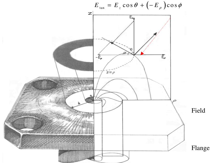
Figure 1: Coaxial line with baffle
